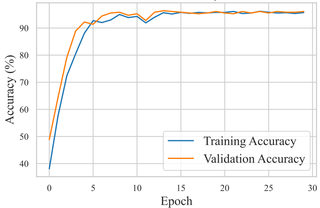
LSTM: Accuracy
