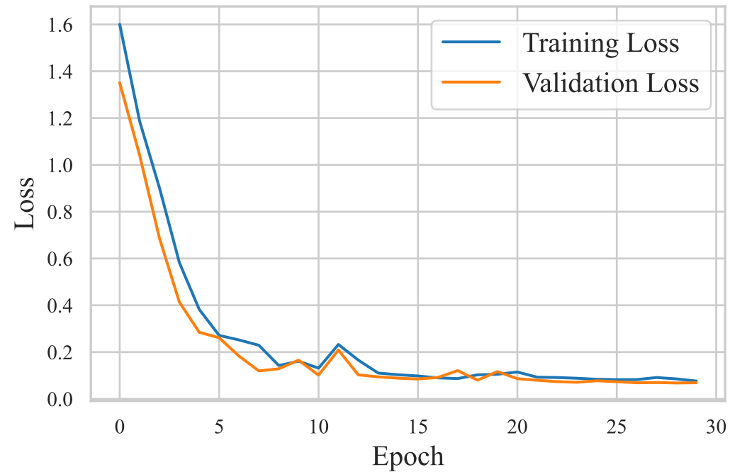
LSTM: Loss
